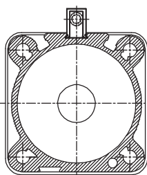
Ø32...Ø100 (DMR)
